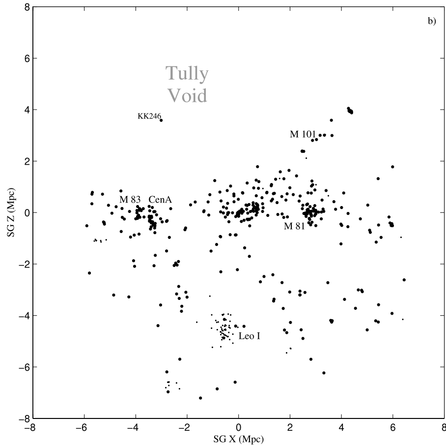
Catalog of Neighboring Galaxies Karachentsev et al. 2004
