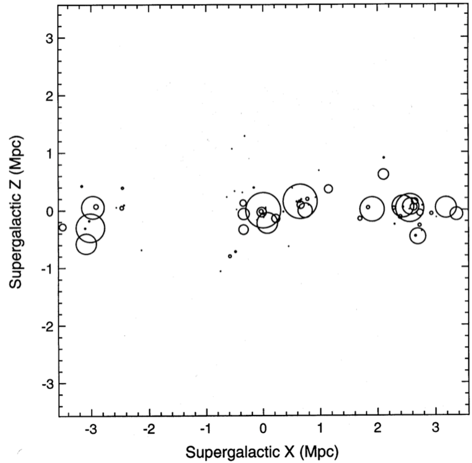
The Local Sheet: X-Side View
