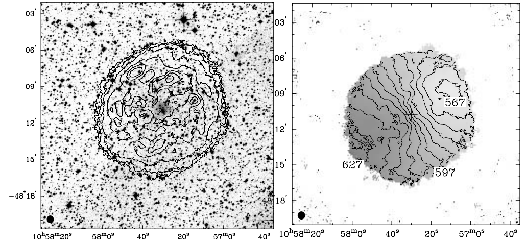
ESO 215-G?009, Warren et al. AJ, 128, 1152 (2004) M_{\text{HI}}/\mathcal{L}_b = 20 M_{\odot}/\mathcal{L}_{\odot} , M_{\text{HI}} = 10^{8.7} M_{\odot} M_{\text{dark}} = 10^{9.6} M_{\odot} within r \sim 7 kpc, v_{\text{escape}} \gtrsim 70 \text{ km s}^{-1}
