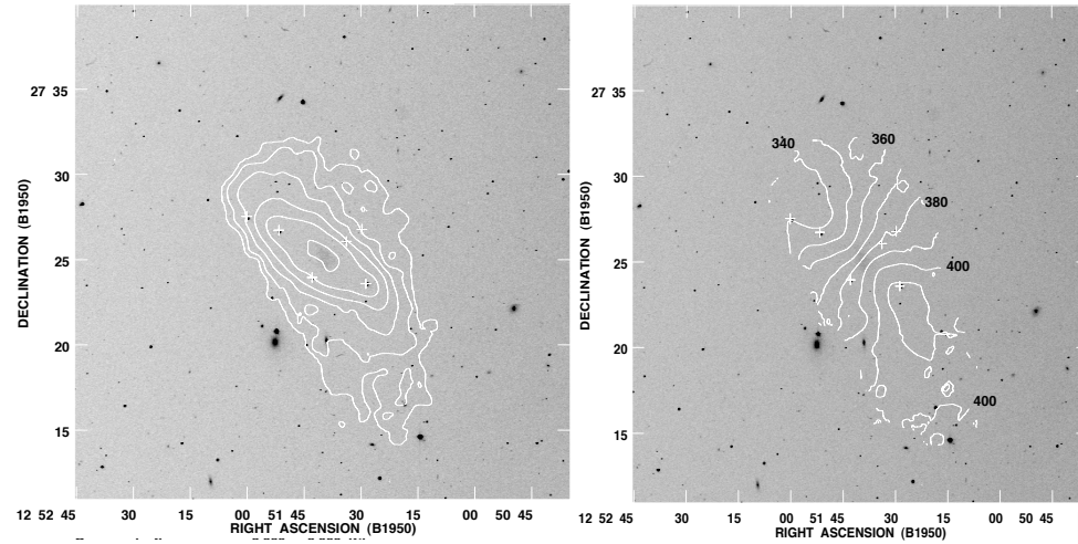
DDO 154 Carignan & Purton (1998) M_{\text{stars}} = 10^{7.6} M_{\odot} , M_{\text{HI}} = 10^{8.4} M_{\odot} M_{\text{dark}} = 10^{9.5} M_{\odot} within r \sim 8 kpc escape velocity \sim 60 \text{ km s}^{-1} from 8 kpc
