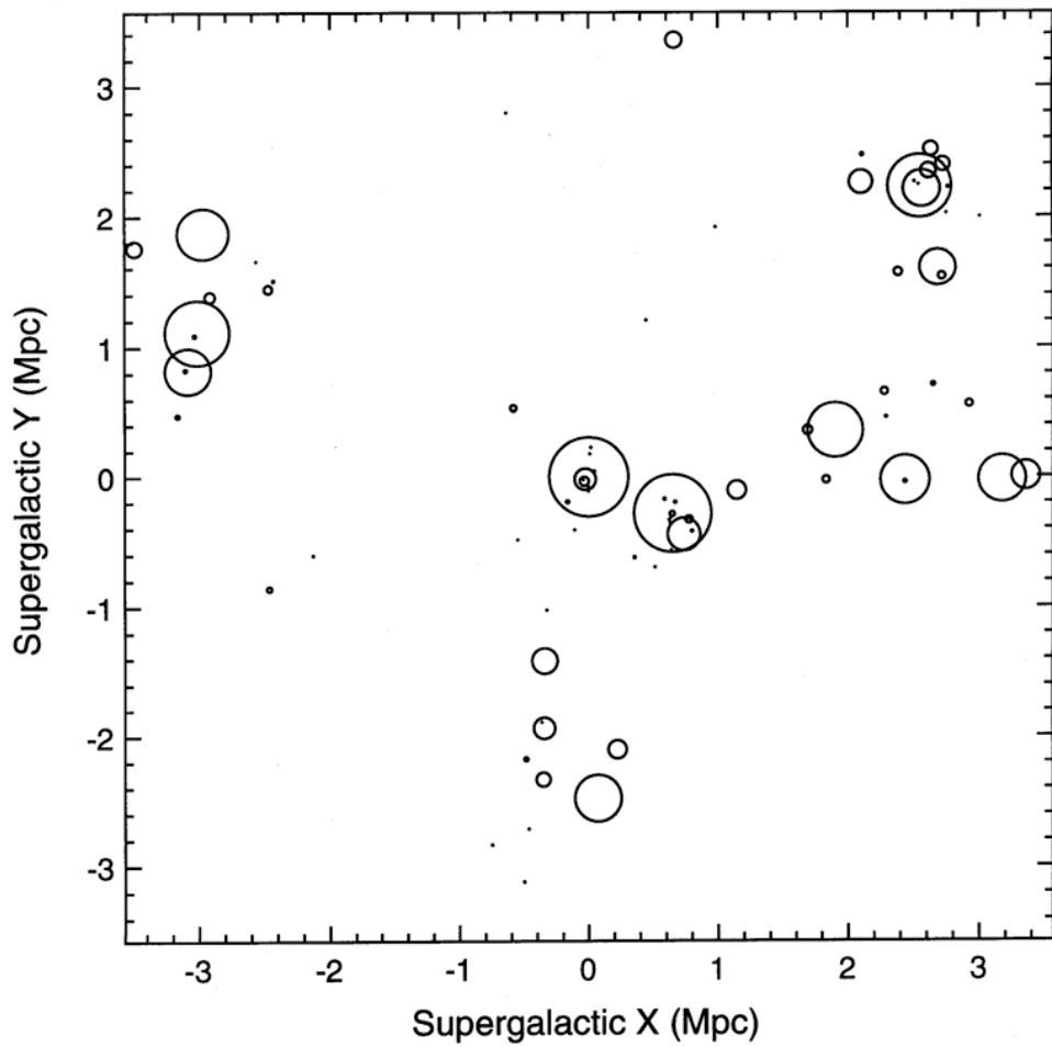
The Local Sheet: Overhead View
