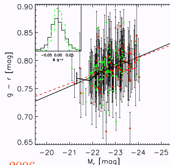
FIG. 8.— Location of C4 BCGs (symbols) with respect to the color-magnitude relation defined by the bulk of the early-type galaxy population (solid line). Dashed line shows a linear fit of color as a function of absolute magnitude, and jagged line with error bars shows the mean color in a few bins in luminosity. Inset shows that BCGs are not offset from the relation defined by the bulk of the popula-
