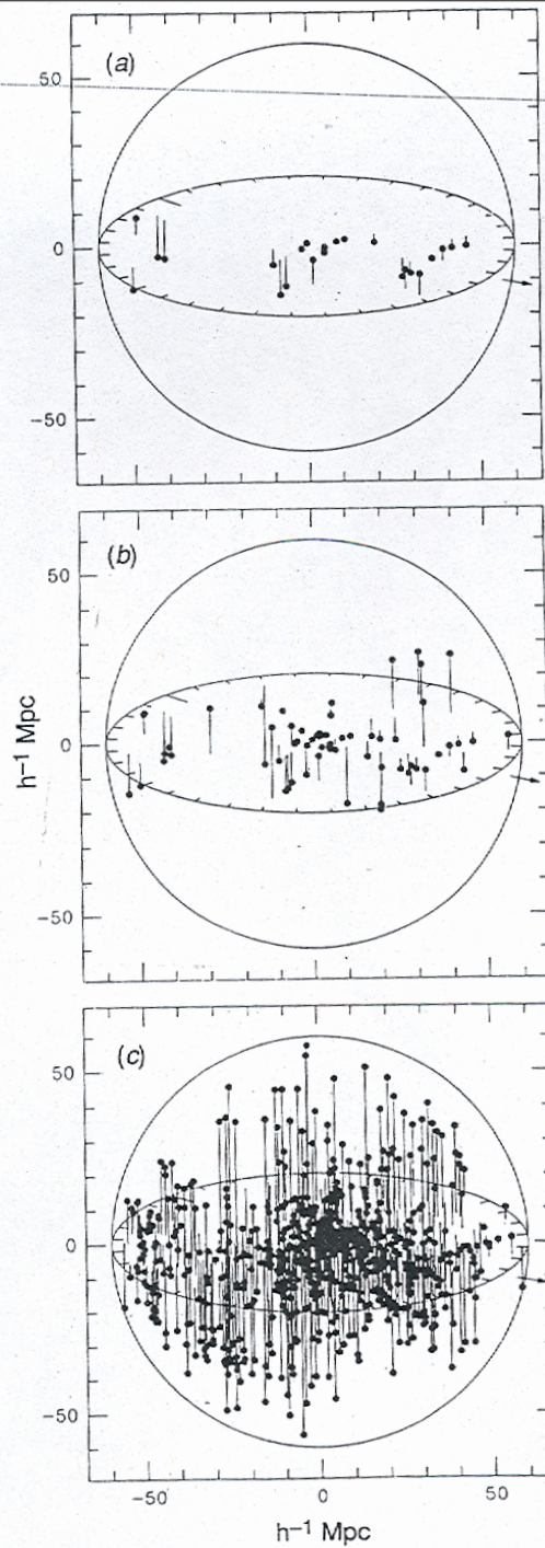
Fig. 5. Space distributions of the complete radio and optical galaxy samples out to z = 0.02 : (a) radio galaxies with S_{408} > 4 Jy, (b) radio galaxies with S_{408} > 1 Jy, and (c) the optical galaxies. Orientation and symbols as in Fig. 4a. The arrows show the 'Great Attractor' direction.
